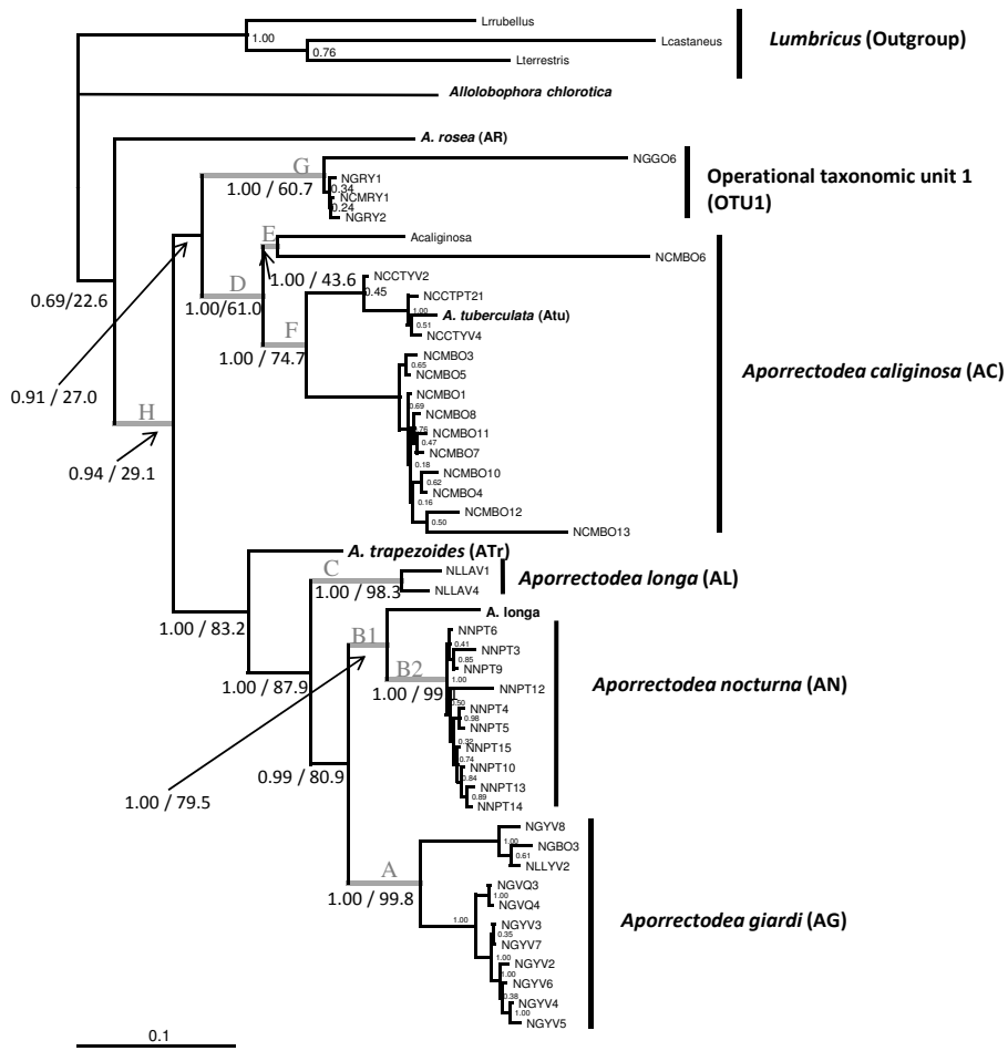
Fig. 1. Phylogenetic relationship obtained from Bayesian Inference analysis on 3 genes concatenated (CO1, 16S & 28S; 1636 nt). Numbers at nodes refer, from left to right respectively, to posterior probabilities in Bayesian analysis and to bootstrap percentages in ML analysis (not shown within species). Dataset was analyzed with the GTR + G model applied to each partition.
