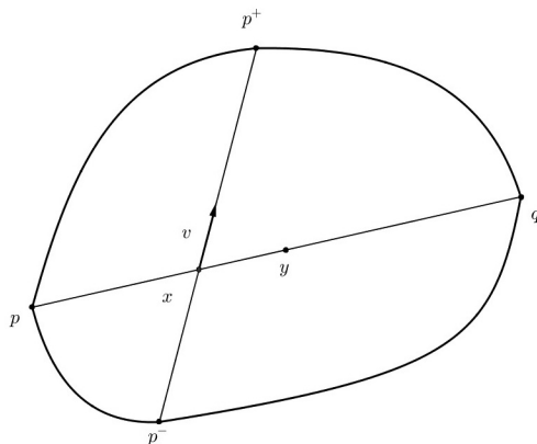
Figure 1. Hilbert distance
