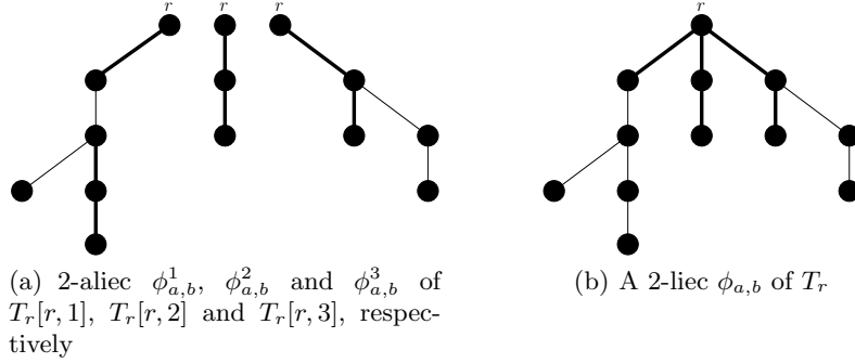
Fig. 1. Examples of rooted trees, shrubs, 2-lic and 2-aliec. Thick (resp. thin) edges represent a -coloured (resp. b -coloured) edges.
