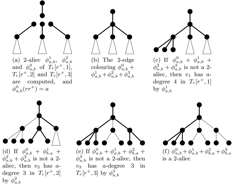
Fig. 2. Application of Algorithm 1 on a shrub T_r such that r^+ has 3 children
