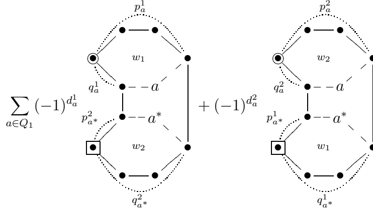
Fig. 2. the graded Kontsevich bracket \{w_1, w_2\} in \mathfrak{n}_Q . The dashed links, the beads inbetween these links (denoted as a and a^* = \frac{\partial}{\partial a} ) and the round ornamentation are removed and the open necklaces are connected as indicated. The exponents used are d_a^1 = (|w_1| - 1)|p_{a^*}^2| + |p_a^1||q_a^1| + 1 and d_a^2 = (|w_2| - 1)|p_a^2| + |p_{a^*}^1||q_{a^*}^1| .
