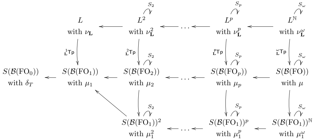
FIGURE 3. Pushforward of measures
