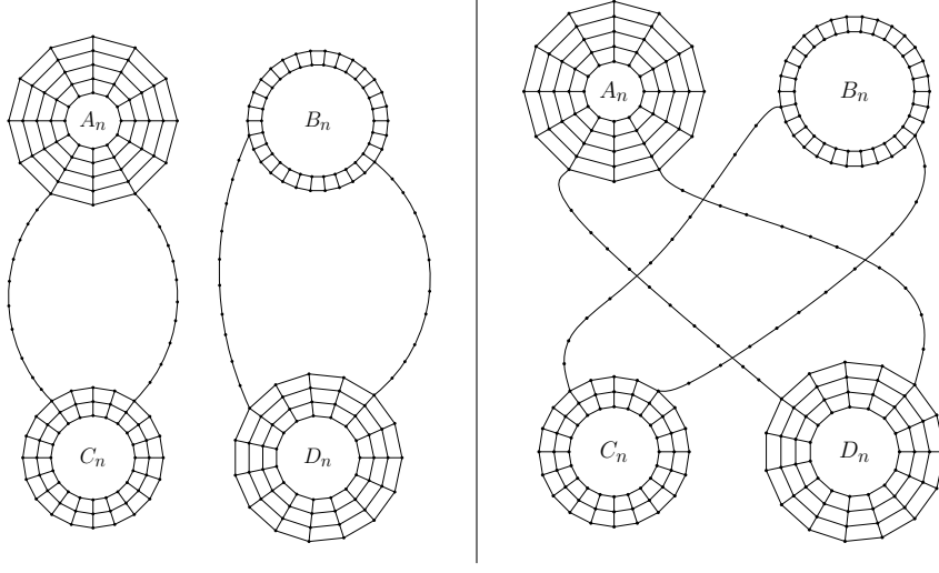
FIGURE 4. An FO-converging sequence with no component selection
