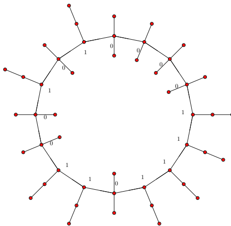
FIGURE 5. The graph G_n is constructed from a De Bruijn sequence of length 2^n .
