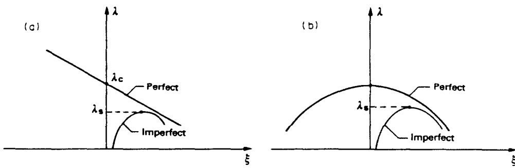
Fig. 1. Equilibrium paths: (a) asymmetric system ( \lambda_1 \neq 0 ); (b) symmetric system ( \lambda_1 = 0, \lambda_2 \neq 0 ).
