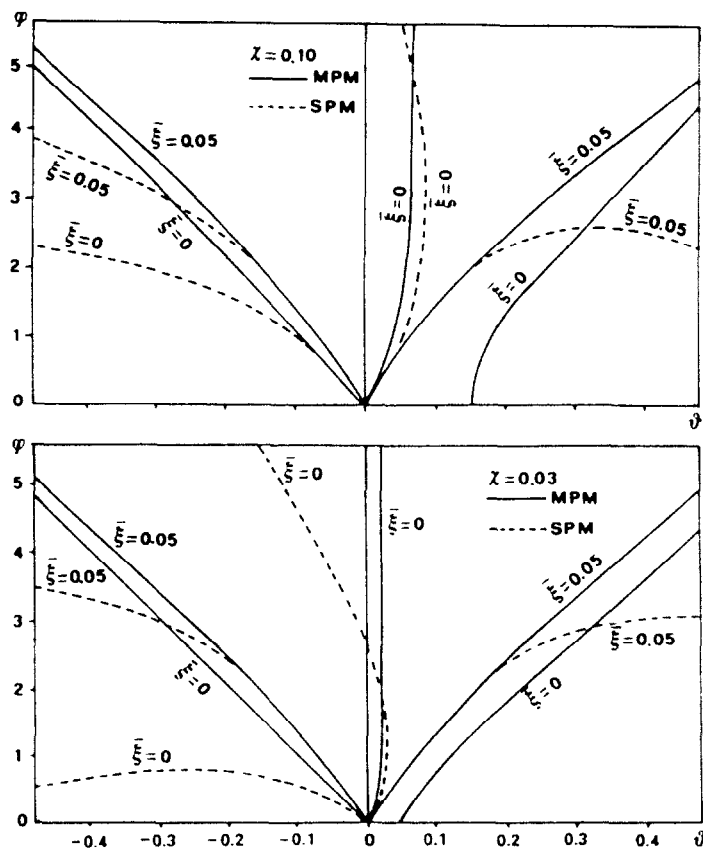
Fig. 7. Equilibrium paths for perfect ( \bar{\xi} = 0 ) and imperfect ( \bar{\xi} = 0.05 ) system.
