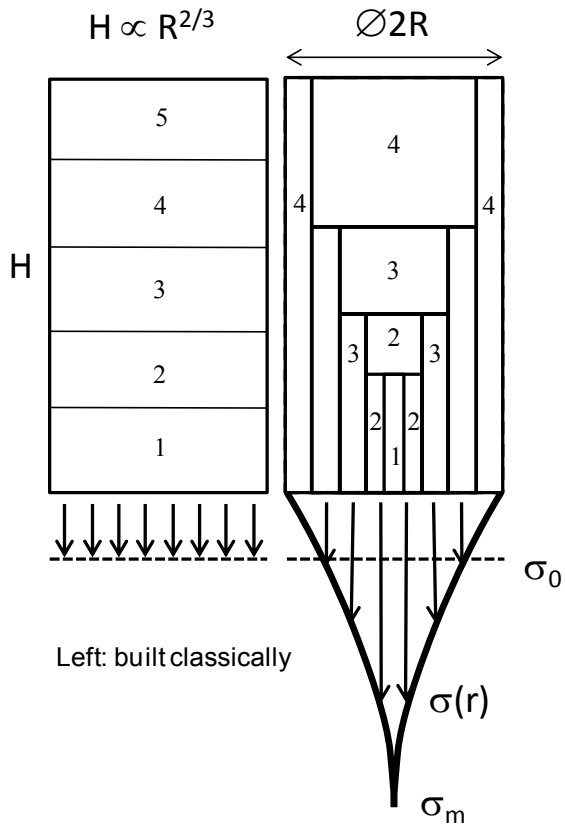
Fig. 1 Compressive support stress distribution at the bottom of a column
