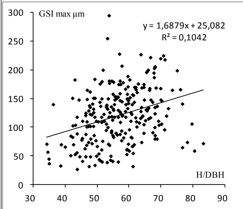
Fig. 7 Relationship between GSI max and H/DBH 251 straight trees
