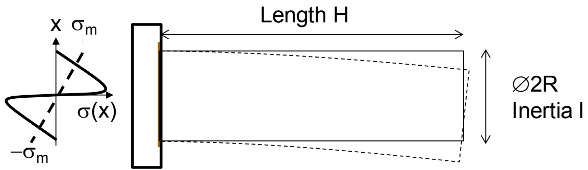
Fig. 2 Stress field on the section of the beam at anchorage level Dotted line: stress distribution for a man-made cylindrical beam Continuous line: stress distribution for a growing stem with constant allometry: H \propto R^{2/3}
