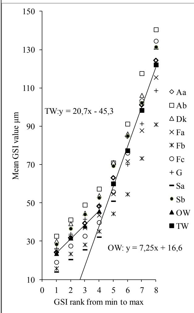
Fig. 8 Eight GSI measurements per tree sorted by value ( Mean per stand) TW: tensile side; OW opposite side
