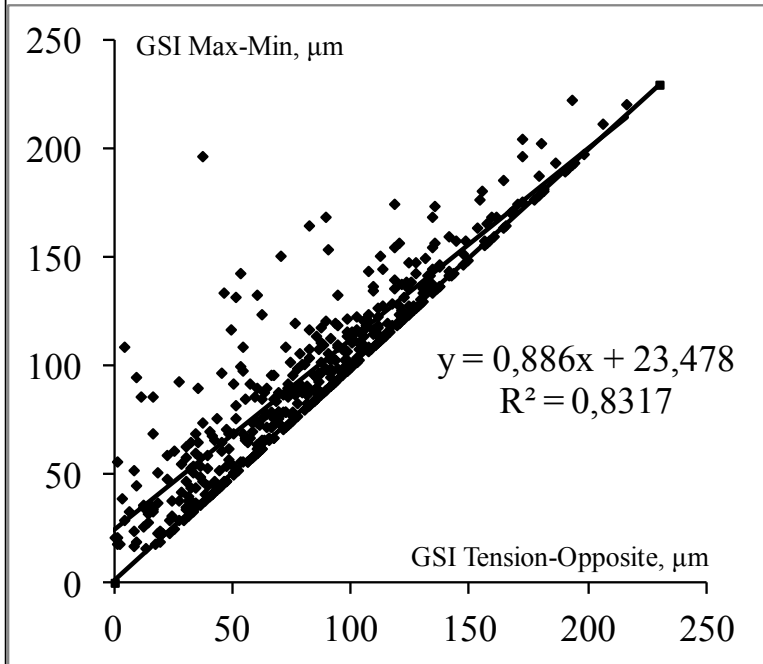
Fig. 6 Relationship between Tension-Opposite Growth Stress Indicator and Max-Min Growth Stress Indicator
