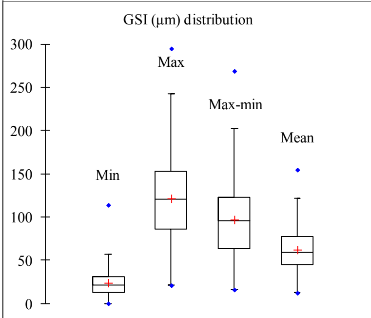
Fig. 5 Distribution of tree Growth Stress Indicator (GSI) parameters 440 trees
