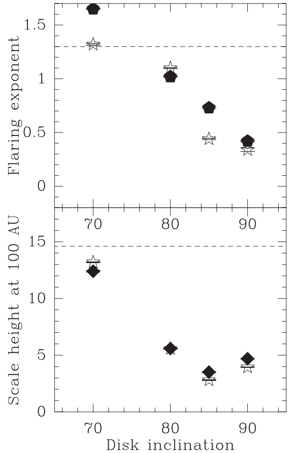
Figure 8. Derived apparent scale heights and flaring index as a function of disk inclination. All results show viscous pseudo-observations (Model 2) fitted by truncated discs (Model 1), using grains of moderate size, with free scale height and radial-dependent \beta (Case 4). Stars show results obtained with the strong dust settling prescription, while filled symbols are obtained with the lowest one. The dashed lines indicate the expected hydrostatic scale height and flaring index for non-settled discs.
