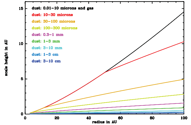
Figure 3. Dust and gas scale heights as a function of the radius for different grain sizes for the settled model. The black curve also corresponds to the gas scale height.
