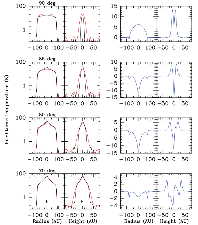
Figure 5. Radial and vertical cuts in brightness temperature distribution (K) of discs with moderate grains, observed at 670 GHz under different inclinations. Left: black curves correspond to the settled model. Red curves correspond to the non-settled model. Right: the differences (non-settled–settled) between these two models are shown in blue. The horizontal bar indicates the angular resolution.
