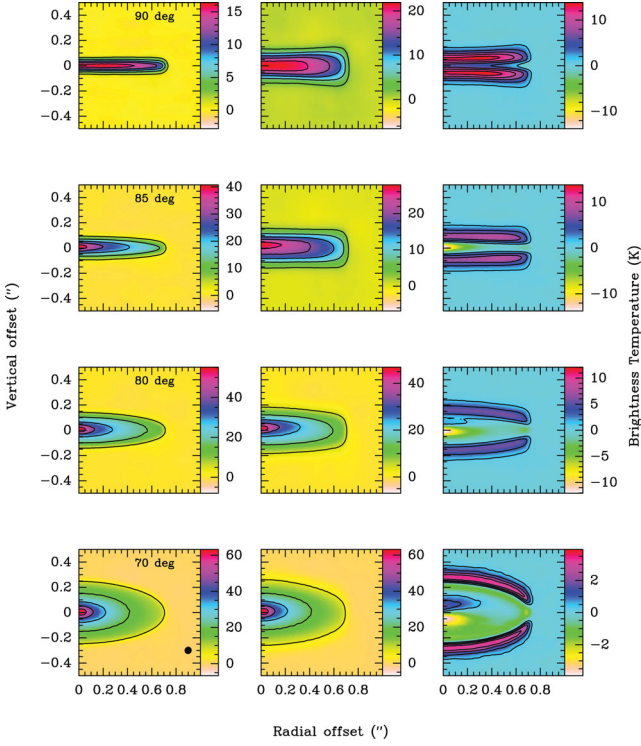
Figure 4. Discs observed at 670 GHz under inclinations of 90°, 85°, 80° and 70°, from top to bottom. Left: settled discs. Middle: non-settled discs of the same gas mass distribution and same amount of dust. Right: difference between these two models (non settled–settled). Simulations are made with moderate grains. The hatched ellipse is the PSF.
