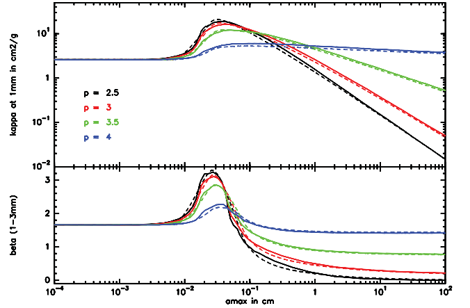
Figure A2. Top panel: absorption coefficient \kappa at 1 mm as a function of a_{\text{max}} for different exponents p of the size distribution. The solid lines represent the results calculated in Ricci et al (2010), using realistic grains made of astronomical silicates (10 per cent in volume), carbonaceous materials (20 per cent) and water ice. The dashed lines represent our approximated method. Bottom panel: emissivity exponent \beta computed between 1 and 3 mm for the same grain distribution.
