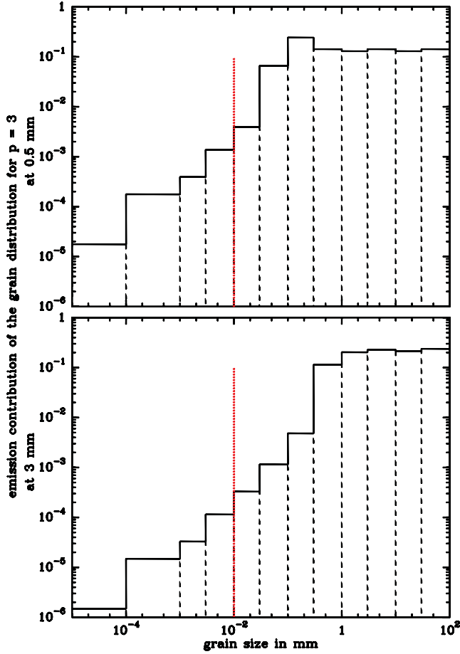
Figure 1. Contribution of various dust grains to the total emission (at 3 and 0.5 mm wavelengths), depending on their size, for an assumed size exponent p_d = 3 . The vertical red dotted line represents approximately (depending on disc density) the separation between grains well mixed with the gas and grains starting to settle.
