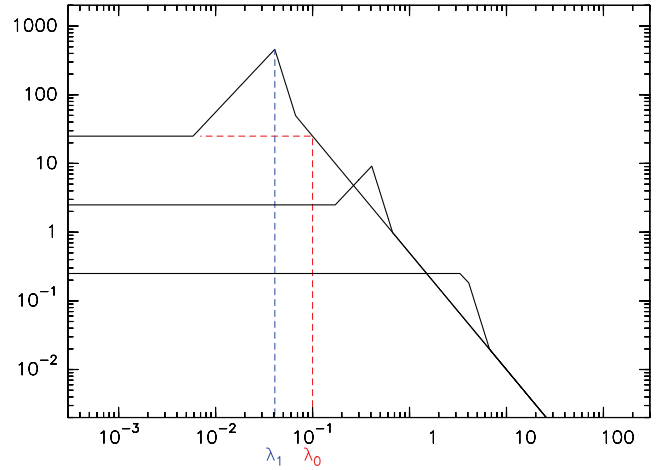
Figure A1. Absorption coefficient as a function \lambda for three different sizes of grains (0.1, 1 and 10 mm). These curves correspond to \rho_d = 1.5 \text{ g cm}^{-3} , long wavelength parameters exponent e_l = -1.7 and coefficient k_l = 0.5 \text{ cm}^{0.3} \text{ g}^{-1} , and bump height f_p = 4 , exponents e_b = 1.5 , e_a = -4.5 and 98 position l_1 = 0.65 .
