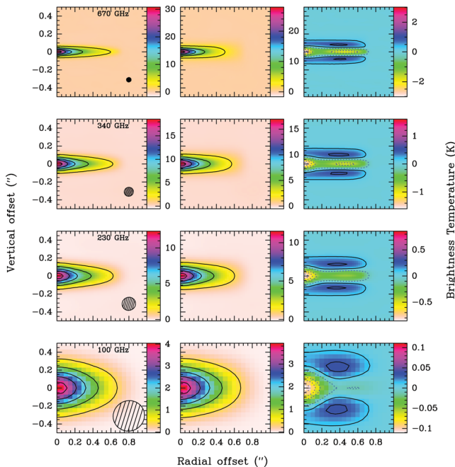
Figure 6. Left: settled discs at 85^\circ of inclination. Middle: results of the best model obtained with the non-settled disc model (Case 1). Right: difference between these two models (non-settled–settled). Models are made with large grains. The hatched ellipse is the PSF.
