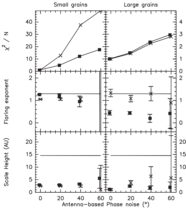
Figure 9. Impact of the phase noise on the measurements of settling. Top: reduced \chi^2 , middle: flaring index h , bottom: apparent scale height at 100 au. Left panels are for the small grain case, and right panels for the big grain case. The truncated power law (model 1) is used. Crosses are for i = 70^\circ , and squares for i = 85^\circ . The horizontal lines indicate the expected values for un-settled discs, derived from the hydrostatic conditions.
