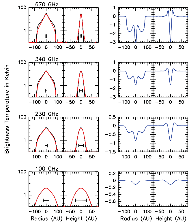
Figure 7. Radial and vertical cuts in brightness temperature distribution (K) at several wavelengths for discs inclined at 85^\circ and large grains corresponding to Fig. 6. Left: black curves correspond to the settled model. Red curves correspond to the non-settled model. Right: the differences (non-settled–settled) between these two models are shown in blue. The horizontal bar indicates the angular resolution.
