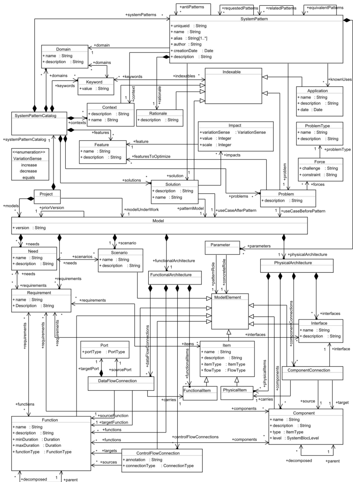
Figure 1. A system-pattern metamodel
