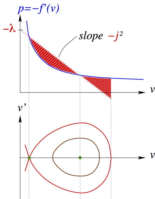
Figure 1: Phase portrait for convex pressure law
