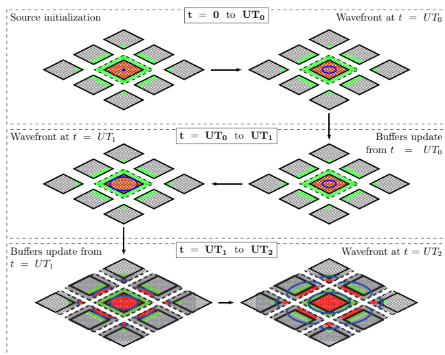
Figure 3: Blocks propagation.
