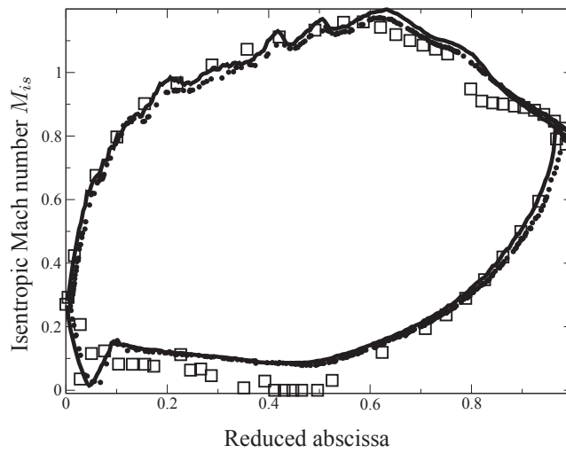
Figure 12 : Isentropic Mach number along the blade. Solid line: coupled LES, circles: adiabatic LES, squares: experiment.
