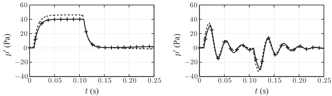
Figure 9 : Time traces of the fluctuating pressure downstream of the nozzle. Numerical results: —; Analytical results: - + -. Left: Non-reflecting case (Analytic compared to Run 2D-1); Right: Finite impedance case (Analytic compared to Run 2D-4).
