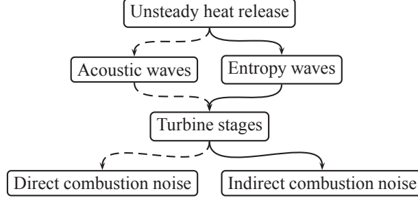
Figure 1 : The two main mechanisms for noise generation from confined flames: direct (---) and indirect (—) noise
