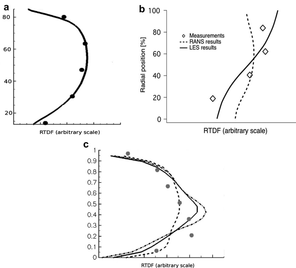
Fig. 27. Outlet normalized temperature profiles (RDTF) obtained numerically by LES, RANS and experiments for different real combustors: (a) Pratt & Whitney engine (LES, line and experiment, symbols) in the plane identified in Fig. 26 [318] (a); (b) Turbomeca engine (LES, RANS and experiment) [319] and (c) Rolls-Royce engine (LES with and without the casing and RANS with the casing) [48]: Symbol, rig measurements; —, LES of liner plus annuli; - -, LES of liner only; and -.-, RANS simulation of liner only.
