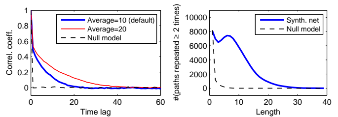
FIG. 5: (color online). Left. Autocorrelation function C(t) vs. t , averaged over 40 realizations of \mathcal{N} , for two distinct walk length averages and compared to a null model where all links have been temporally randomized, equivalent to imposing that all walks in the construction have length 1. Right. Number of \tau -tolerant temporal paths ( \tau = 5 ) occurring at least twice vs. their length, both in \mathcal{N} and in the null model.
