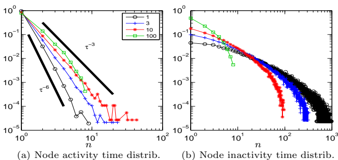
FIG. 4: (color online). Distributions of activity (a) and inactivity (b) periods aggregated over intervals of various lengths T_{\text{agg}} = 1, 3, 10, 100 , i.e. fractions of nodes that are active at least once in each of (resp. inactive during) n consecutive intervals of duration T_{\text{agg}} (the maximal value of n is T/T_{\text{agg}} ).
