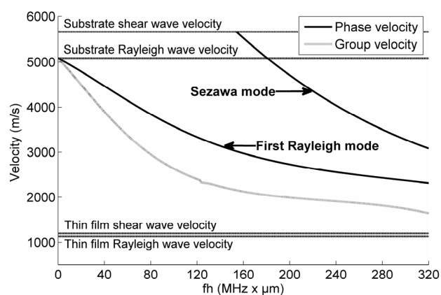
FIG. 2. Rayleigh modes dispersion curves for 2 \mu\text{m} gold thin film deposited on a silicon substrate.
