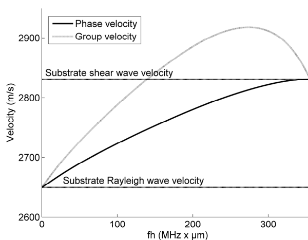
FIG. 1. Rayleigh mode dispersion curves for 2 \mu\text{m} silicon thin film deposited on a zinc oxide substrate.
