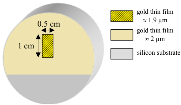
FIG.6. Studied sample layout.
