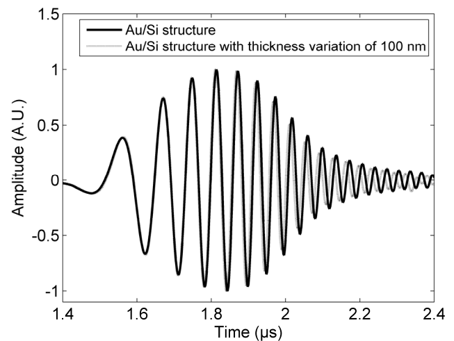
FIG.9. First Rayleigh mode on Au/Si structure and on Au/Si structure with thickness variation.
