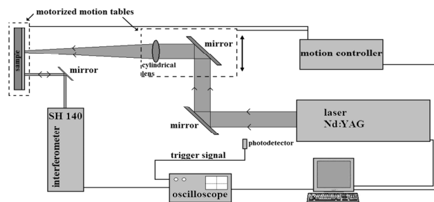
FIG.7. Laser-ultrasonics setup.
