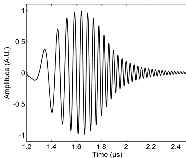
FIG.4. Normal displacement associated with the first Rayleigh mode obtained for a 2 \mu\text{m} gold thin film deposited on a silicon substrate.
