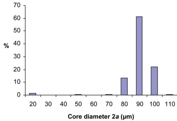
Figure 3. Histogram of the diameters of PMMA particles. [Color figure can be viewed in the online issue, which is available at wileyonlinelibrary.com .]
