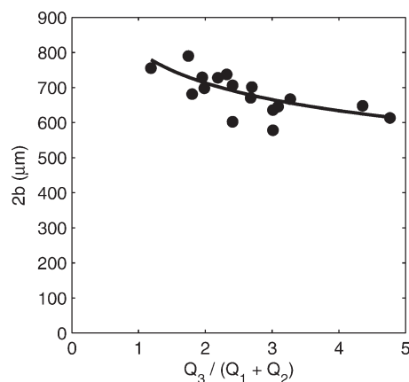
Figure 11. Evolution of the outer diameter of the core shell particles as a function of the flow rate ratio. The continuous line is the best fit of the data to a power law and leads to 2b \sim [Q_3 / (Q_1 + Q_2)]^{0.17} .
