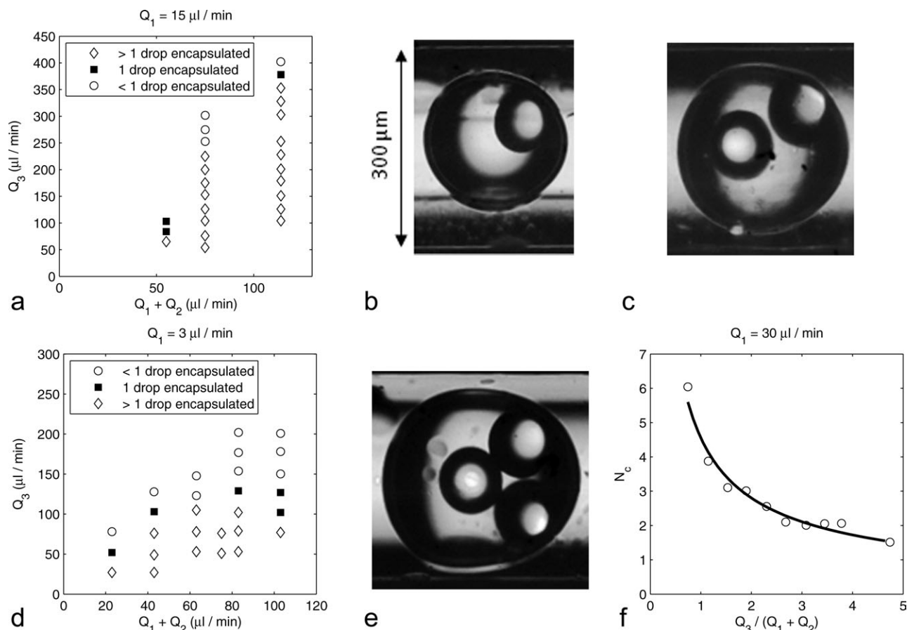
Figure 10. Flow diagrams of the encapsulation stage of the C2 E2 route in the drop only region as functions of internal ( Q_1 + Q_2 ) and external ( Q_3 ) flow rates for (a) Q_1 = 15 \mu\text{L/min} , (d) Q_1 = 3 \mu\text{L/min} . (b) Capsule with two cores obtained for Q_1 = 3 \mu\text{L/min} , Q_2 = 40 \mu\text{L/min} , and Q_3 = 75 \mu\text{L/min} . (c) Capsule with a single core obtained for Q_1 = 3 \mu\text{L/min} , Q_2 = 40 \mu\text{L/min} , and Q_3 = 100 \mu\text{L/min} . (e) Capsule with three cores obtained for Q_1 = 15 \mu\text{L/min} , Q_2 = 60 \mu\text{L/min} , and Q_3 = 125 \mu\text{L/min} . (f) Variation of the average number of EGDA cores per capsule as a function of the imposed flow ratio for Q_1 = 30 \mu\text{L/min} . The solid curve is the best fit of the data set to a power law and leads to N_c \sim [Q_3 / (Q_1 + Q_2)]^{0.7} .
