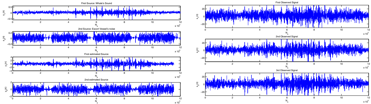
Figure 7 Experimental results: first column contains the original and the estimated sources, and second column contains the observed signals, (the sources are: whale sound and a boat noise).
