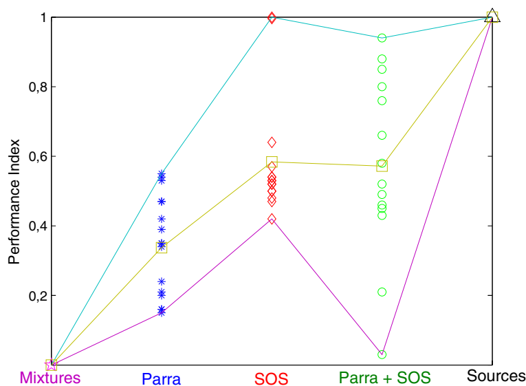
Figure 8 Experimental results obtained by different algorithms, (Parra, SOS or SOS + Parra), on divers configurations and using a normalized performance index (here the three curves represent maximum, minimum and average performance levels). Further details are given in Section “Experimental results”.
