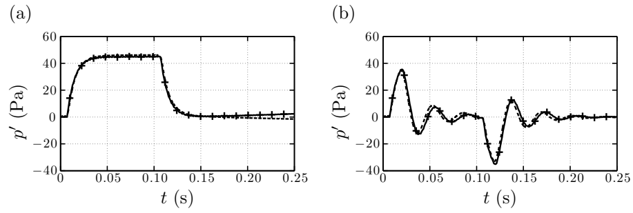
Figure 13: Time traces of the fluctuating pressure 350 mm downstream of the nozzle. Numerical results: ---- ; Analytical results with reflections at the inlet and \ell_{\text{out}} = 2100 mm: -+- . (a) Non-reflecting case (Analytic compared to Run 2D-1); (b) Finite impedance case (Analytic compared to Run 2D-4).
