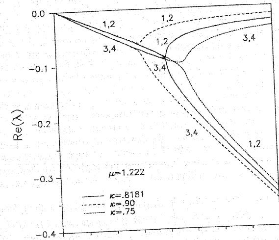
Fig. 5 Eigenvalues vs damping modifications.
