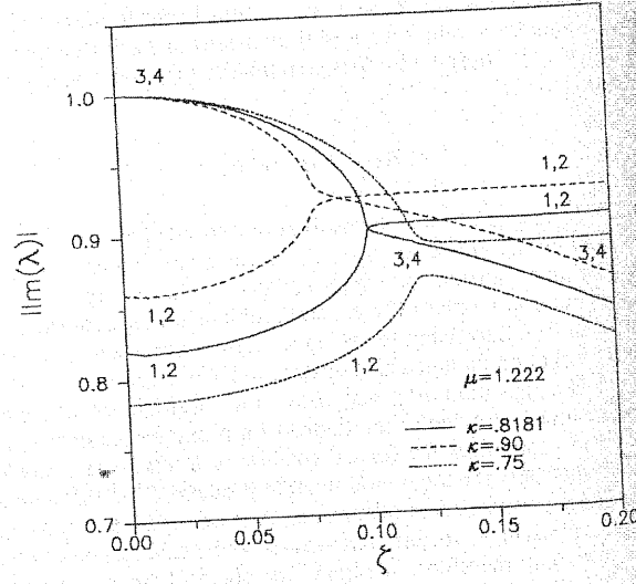
Fig. 5 Eigenvalues vs damping modifications.
