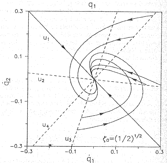
Fig. 4 Critically damped system motions: a) configurations plane and b) velocities plane.
