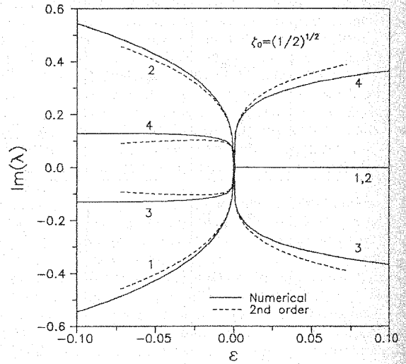
Fig. 9 Eigenvalues vs parameters modifications: critically damped system.
