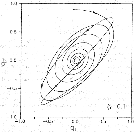
Fig. 2 Underdamped system: a) amplitude-decaying periodic motion and b) nonperiodic motions.
