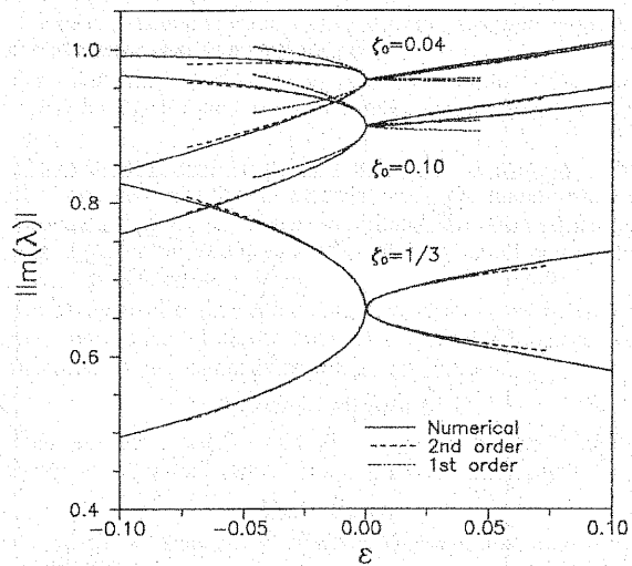
Fig. 7 Eigenvalues vs parameters modifications: underdamped systems.
