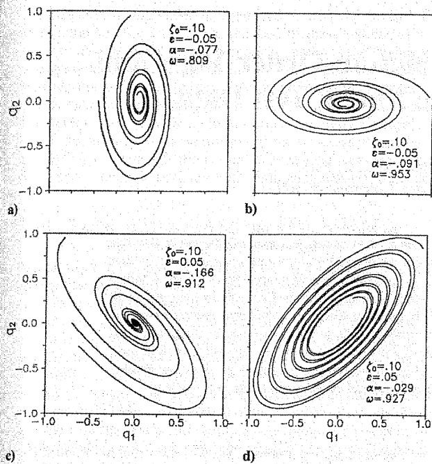
Fig. 11 Amplitude-decaying periodic motions of an underdamped oscillator.
