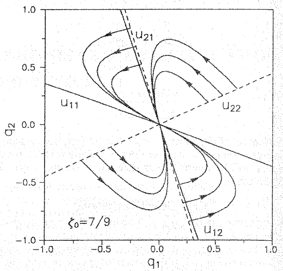
Fig. 3 Overdamped system motions.
