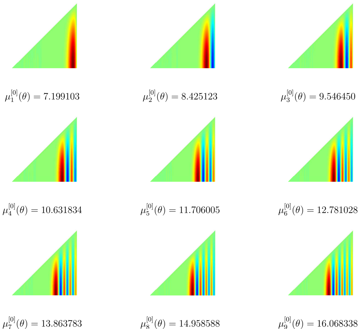
Figure 7: Computation for \theta = 0.0226 * \pi/2 \sim 2^\circ . Numerical values of the nine first eigenvalues for m = 0 . Plots of the associated eigenfunctions in the domain \text{Tri} .
