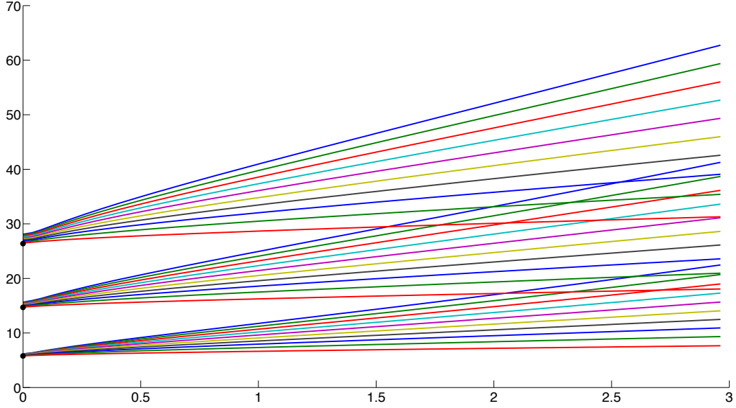
Figure 3: This figure represents the dependence of the first ten eigenvalues \lambda_n^{[m]}(\tan \theta) ( m = 0, 1, 2 ) on the aperture \theta (in degrees). We computed each eigenvalue for 80 values of \theta .
