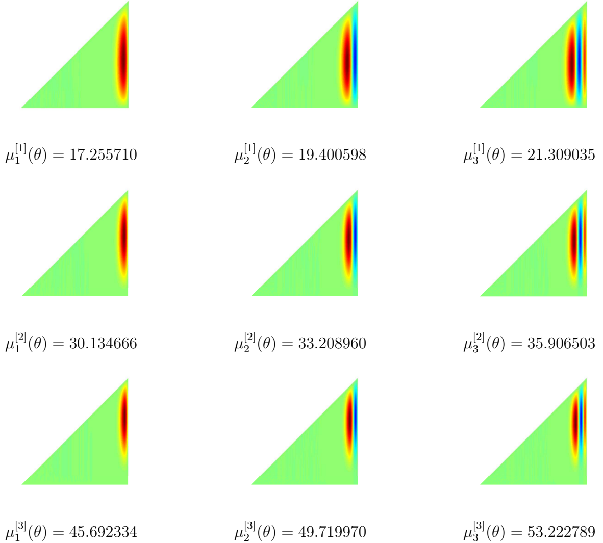
Figure 8: Computation for \theta = 0.0226 * \pi/2 \sim 2^\circ . Numerical values of the three first eigenvalues for m = 1 , m = 2 and m = 3 . Plots of the associated eigenfunctions in the meridian domain Tri.
