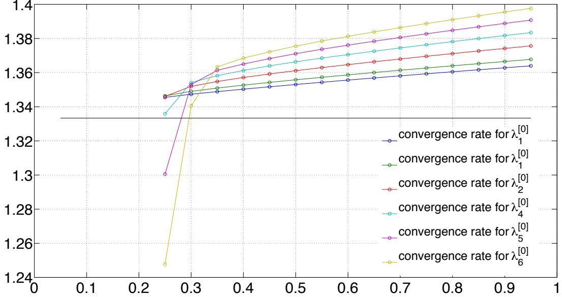
Figure 4: This figure represents the convergence rate of the first six eigenvalues \lambda_n^{[0]}(\tan \theta) to the two first terms of the theoretical asymptotics on the aperture \theta (in degrees). The black line represents the value 4/3 .
