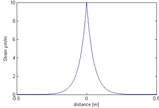
Figure 3: Mechanical Transfer Function of a commercial cable [6]
