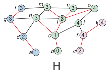
Fig. 65. Flooding from the minima of a node weighted graph controlled by a hierarchical queue. The nodes in the queue have two colors : the already expanded nodes are in dark blue and the nodes still to expand are in red. The lexicographic distance of each package of nodes is placed above the package.
