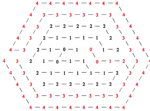
Fig. 21. Edge weights produced by the dilation \delta_{en} of the hexagonal distance function on a small portion of the image.
