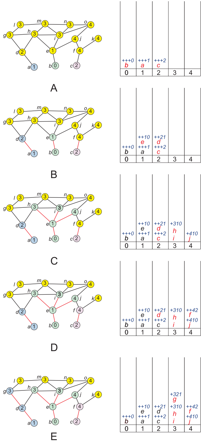
Fig. 64. Flooding from the minima of a node weighted graph controlled by a hierarchical queue. The nodes in the queue have two colors : the already expanded nodes are in dark blue and the nodes still to expand are in red. The lexicographic distance of each package of nodes is placed above the package.
