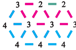
Fig. 21. Edge weights produced by the dilation \delta_{en} of the hexagonal distance function on a small portion of the image.
