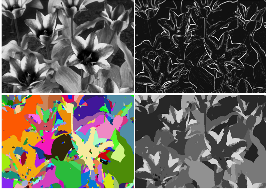
Fig. 46. Initial image, gradient, labeled regional minima and as final result the catchment basins containing each the mean gray tone of the initial image.
