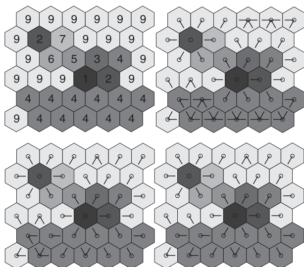
Fig. 43. Successive prunings of the arrows.
