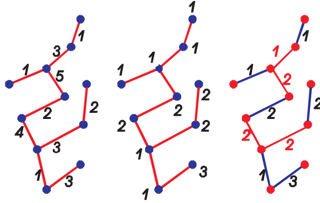
Fig. 11. From left to right: 1) an edge weighted graph, in the centre, 2) the result of the erosion \varepsilon_{ne} , 3) the subsequent dilation produces an opening. The edges in red are those whose weight has been reduced by the opening as they were not the lowest edge of one of their extremities in the initial distribution of edge weights.
