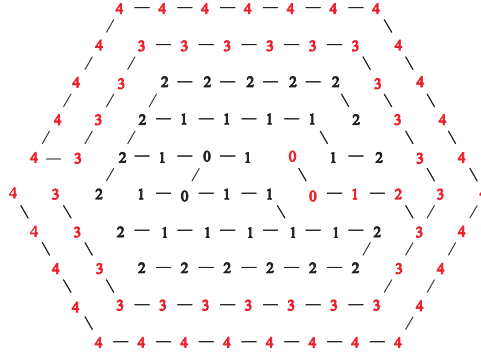
Fig. 21. Edge weights produces by the dilation \delta_{en} of the hexagonal distance function on a small portion of the image.
