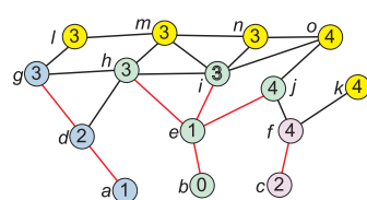
Fig. 64. Flooding from the minima of a node weighted graph controlled by a hierarchical queue. The nodes in the queue have two colors : the already expanded nodes are in dark blue and the nodes still to expand are in red. The lexicographic distance of each package of nodes is placed above the package.
