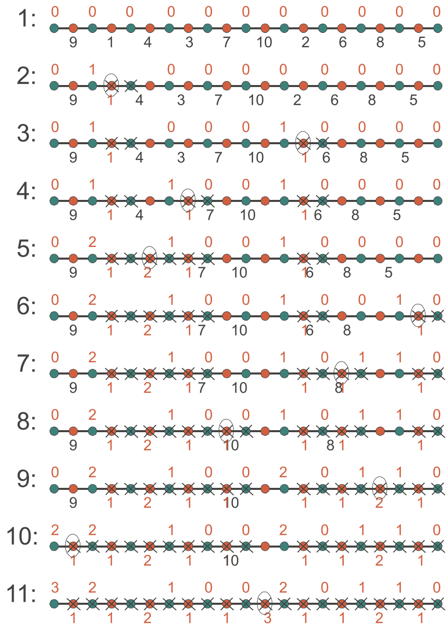
Fig. 30. Construction of the waterfall hierarchy in one run
