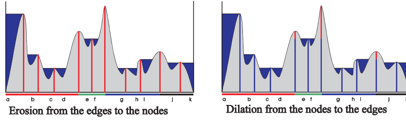
Fig. 10. On the left: waterfall flooding by an erosion between edges and nodes ; on the rights subsequent dilation between nodes and edges yielding an opening.
