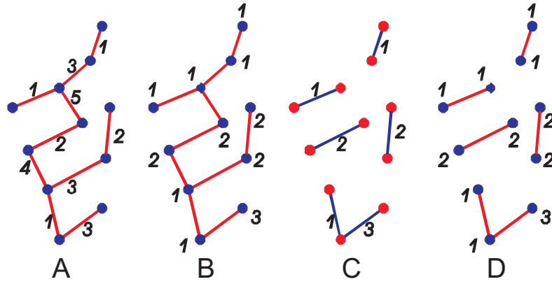
Fig. 13. A: Initial edge weighted graph G B: Erosion \varepsilon_{ne} from the edges to the nodes on G C: The graph \downarrow G D: Erosion \varepsilon_{ne} from the edges to the nodes on \downarrow G : \varepsilon_{ne}(G) = \varepsilon_{ne}(\downarrow G)
