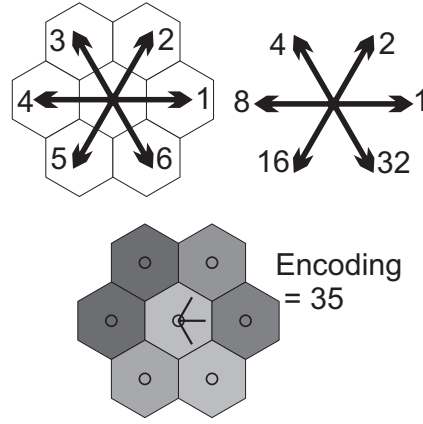
Fig. 31. The encoding of the directions of the neighbors in the hexagonal raster, and the weights of the corresponding bits in the binary representation of the arrows. An example with three arrows with weights 2, 1 and 32 is represented by the binary number 100011, i.e. the decimal number 35.
