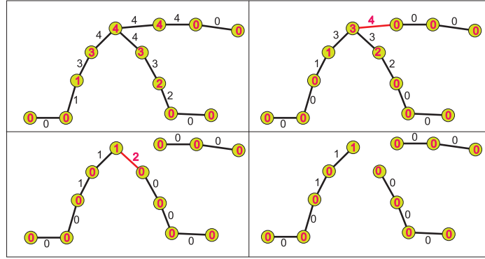
Fig. 60. Successive prunings of a graph when one applies the series \zeta^{(n)}G
