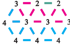
Fig. 21. Edge weights produces by the dilation \delta_{en} of the hexagonal distance function on a small portion of the image.
