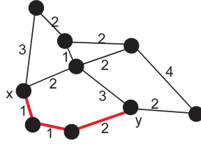
Fig. 4. The shortest chain (sum of the weights of the edges) between x and y is a red line and has a length of 4. It is also the lowest chain (maximum of the weights of the edges) with a maximal weight of 2.
