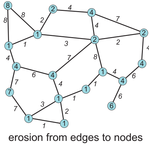
Fig. 8. The edge weights are given and the node weights are the result of the erosion between edges and nodes
