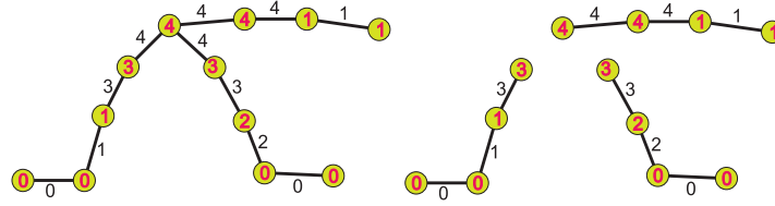
Fig. 57. Lexicographic distance of depth 1.
