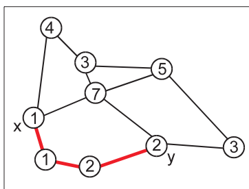
Fig. 6. The cheapest chain between x and y is in red and the total toll to pay is 1 + 1 + 2 + 2 = 6 .
