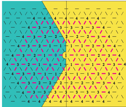
Fig. 24. 2-step flooding graph, obtained by keeping only the edges linking each node with its lowest neighbors.
