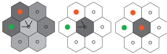
Fig. 39. In the case where two or more distinct labels are present in the direction of arrows, the highest of them, or one, chosen arbitrarily, is propagated
