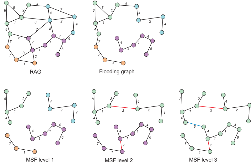
Fig. 29. An edge weighted graph, its floodign graph, and the minimum spanning forests at 3 waterfall hierarchical levels.
