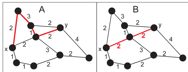
Fig. 5. Lexicographic distances. The toughness of the red chain in fig.A in the direction from x to y is [3, 2] : after crossing the highest edge at altitude 3, the next highest edge has altitude 2. The easiest chain from x to y it indicated in red in fig.B, its toughness is [2, 2] .
