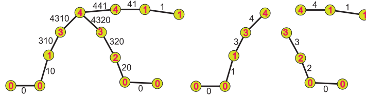
Fig. 59. Lexicographic distance of depth 3.
