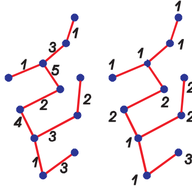
Fig. 7. On the left an edge weighted graph. On the right the result of the erosion between edges and nodes.
