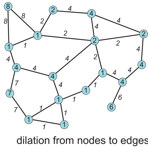
Fig. 9. The node weights are given and the edge weights are the result of the dilation between edges and nodes
