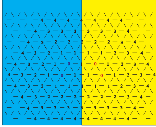
Fig. 20. Hexagonal distance function to two binary sets.
