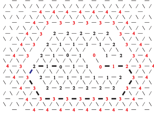
Fig. 23. two flooding tracks leading to the regional minima.
