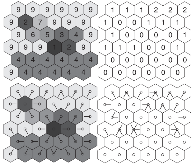
Fig. 44. Top: On the left a topographic surface and on the right the geodesic distance to its lower boundary on each plateau. Bottom: On the left the arrows of the steepest drainage graph and on the right the arrows associated to the distance function.
