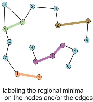
Fig. 18. As the minima are identical on the nodes or the edges of a flooding graph, it is possible to assign the same labels to nodes or to edges.
