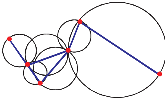
Fig. 3. Two points p and q are connected if there is no third point falling in a disk of diameter pq .
