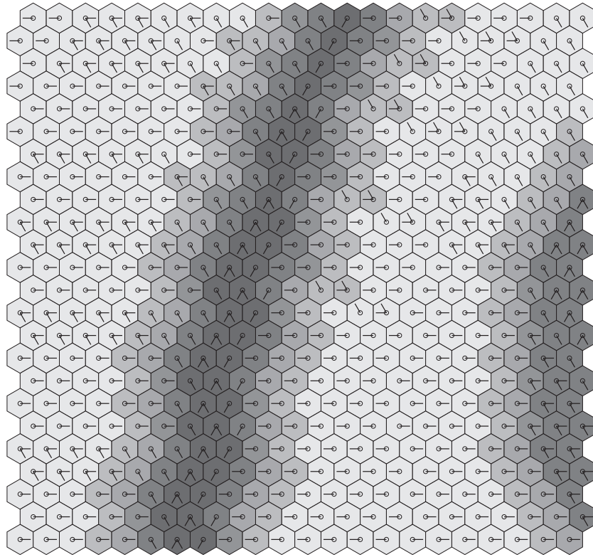
Fig. 53. The arrows of the steepest drainage graph after constructing the geodesic distance of each node of a plateau to the lower border of the plateau.
