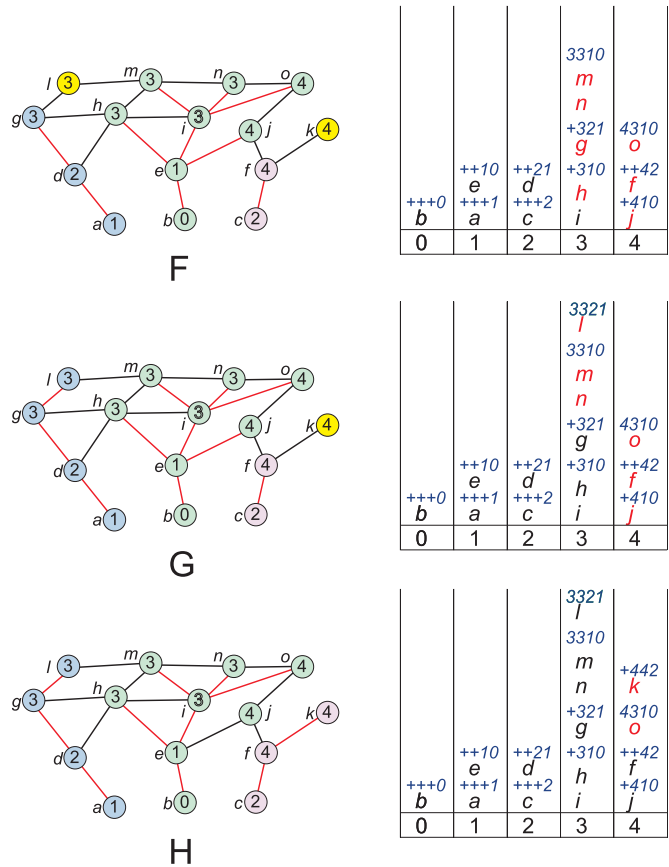
Fig. 65. Flooding from the minima of a node weighted graph controlled by a hierarchical queue. The nodes in the queue have two colors : the already expanded nodes are in dark blue and the nodes still to expand are in red. The lexicographic distance of each package of nodes is placed above the package.
