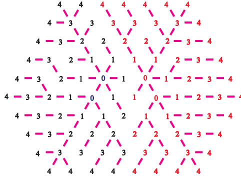
Fig. 25. A minimum spanning forest produced by the operator \chi \Downarrow = \chi \downarrow^2
