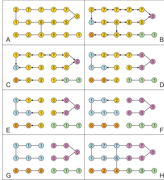
Fig. 19. Construction of the catchment basins of a node weighted graph
