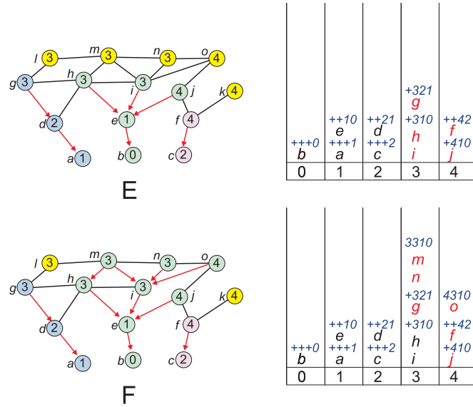
Fig. 66. Arcs are created between each flooded node and its smallest flooding nodes, in the sense of the lexicographic distance of depth \infty .
