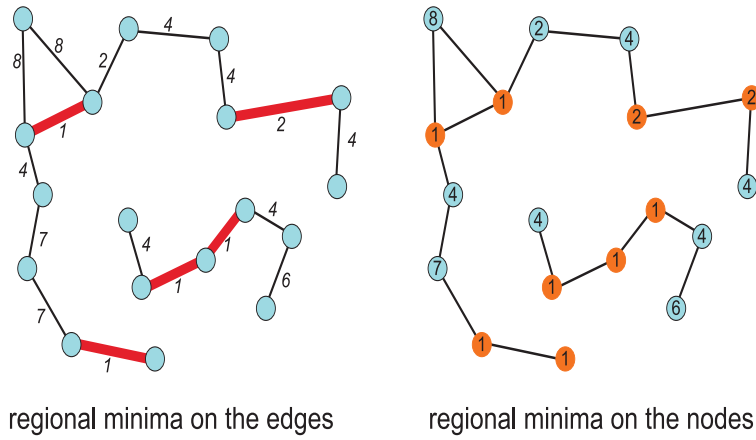
Fig. 17. Whether one consider the egde weights or the node weights produces the same regional minima.
