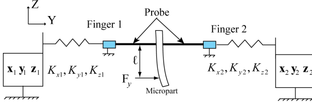
Fig. 7. Microgripper model based on two-sensing-finger microgripper.
