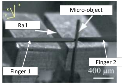
Fig. 23 Guiding task: a micro-object is held between two fingers of a microgripper and guided in the rail
