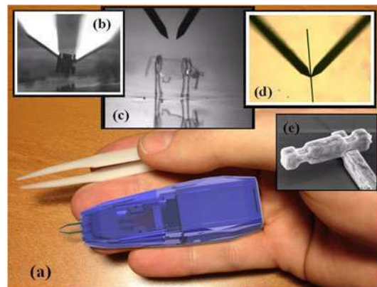
Fig. 7 a PiTweez from PERCIPIO-ROBOTICS, b micromanipulation of a silicon micro part 40 \mu\text{m} \times 40 \mu\text{m} \times 5 \mu\text{m} , c polymer micro-cow to demonstrate micro-assembly (500 \mu\text{m} long, smallest nose part is 50 \mu\text{m} \times 50 \mu\text{m} \times 5 \mu\text{m} ), d fiber, 7 \mu\text{m} diameter, e silicon parts assembly, 7 \mu\text{m} width
