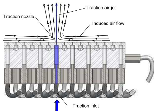
Fig. 12 The induced air flow surface
