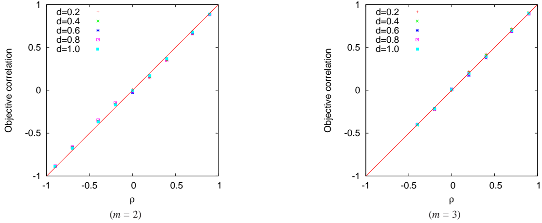
Figure 2: Average value of the Spearman correlation coefficient between the objective function values and the correlation coefficient \rho . The decision space is enumerated exhaustively for n = 18 on a set of 30 independent random instances. The number of objectives is m = 2 (left) and m = 3 (right).
