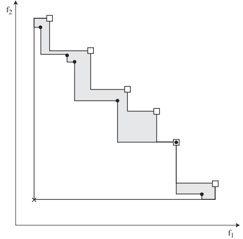
Figure 7: Illustration of the hypervolume difference quality indicator ( I_H^- ). The reference set is represented by boxes ( \square ), the Pareto front approximation by bullets ( \bullet ) and the reference point z^l by a cross ( \times ). The shaded area represents the hypervolume difference I_H^-(\bullet, \square) .
