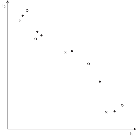
Figure 6: Illustration of the Pareto dominance relation over Pareto front approximations: (i) the approximation (•) dominates the approximation (x), (ii) the approximations (•) and (o) are incomparable, and (iii) the approximations (x) and (o) are incomparable.
