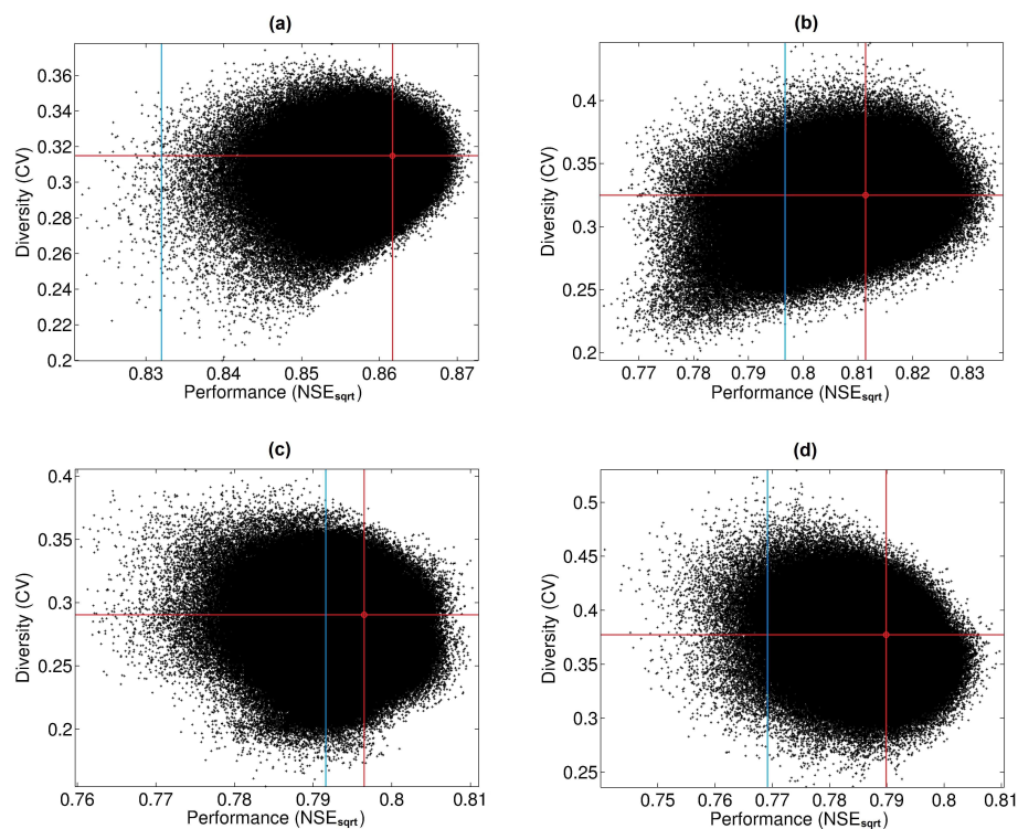
Fig. 11. Validation performance ( NSE_{sqrt} ) and diversity (CV) for all model combinations ( 2^{20} points) and Differential Split Sample Tests for the Au Saumon catchment (SAU): (a) calibration on DW years (dry/warm) and validation on HC years (humid/cold); (b) calibration on HC years (humid/cold) and validation on DW years (dry/warm); (c) calibration on DC years (dry/cold) and validation on HW years (humid/warm); (d) calibration on HW years (humid/warm) and validation on DC years (dry/cold). Red lines and circle illustrate performance and diversity of the twenty-member ensembles and blue lines, of the best individual model for each test.
