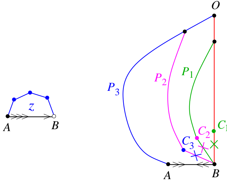
Fig. 12: Inductive definition of the bijection between d -irreducible k -slices and d -oriented k -trees. Left: the (d - 2) -slice reduced to a single inner face is associated with the (d - 2) -tree reduced to a single leaf edge. Right: given a k -slice of size > 1 , we perform its iterated decomposition: the corresponding k -tree is obtained by keeping the root edge AB , which we decorate into an edge of type k/(d - 1 - k) , and then inductively constructing the trees associated with the subslices delimited by P_1, P_2, \dots (thus the edges BC_1, BC_2, \dots will be kept in the tree at the next stage).
