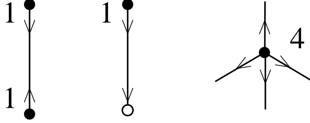
Fig. 14: The rules of Fig. 11 in the particular case d = 3 . The out-degree of all inner vertices is always 1, so that inner vertices have necessarily degree 4. We deduce that 3-oriented 1-trees reduce to ternary trees.
