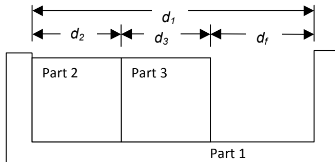
Figure 2. A simple 1-dimensional example showing tolerance analysis with only dimensional tolerances.
