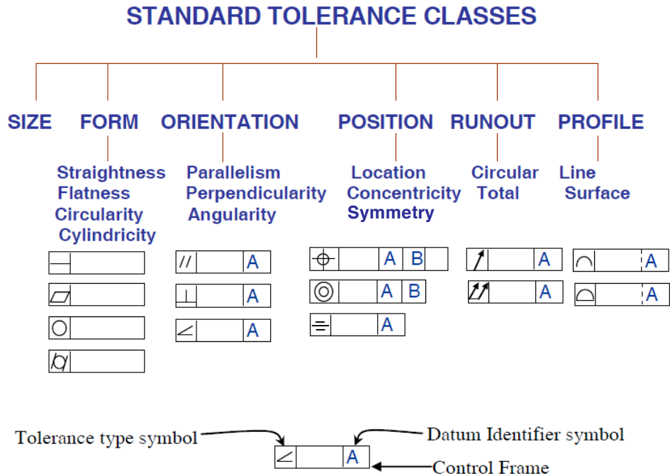
Figure 1: Different classes of tolerances in the standards [1].
