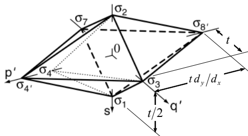
Figure 5. The T-Map for the tolerance zone shown in Figure 4(c).
