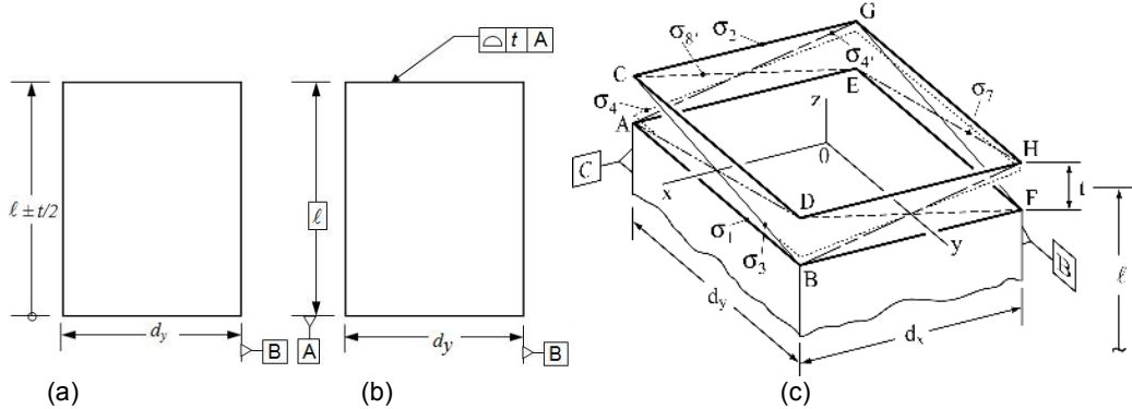
Figure 4. (a) Rectangular part with size tolerance and (b) rectangular part with profile tolerance on rectangular surface. (c) The tolerance zone on size (specification of (a)) or profile (specification of (b)) for a rectangular bar and a coordinate frame centered within it.
