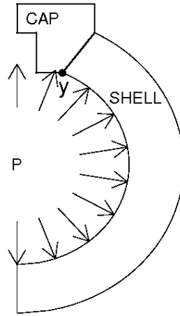
Figure 2. Tank distortion at point y
