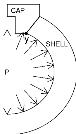
Figure 2. Tank distortion at point y
