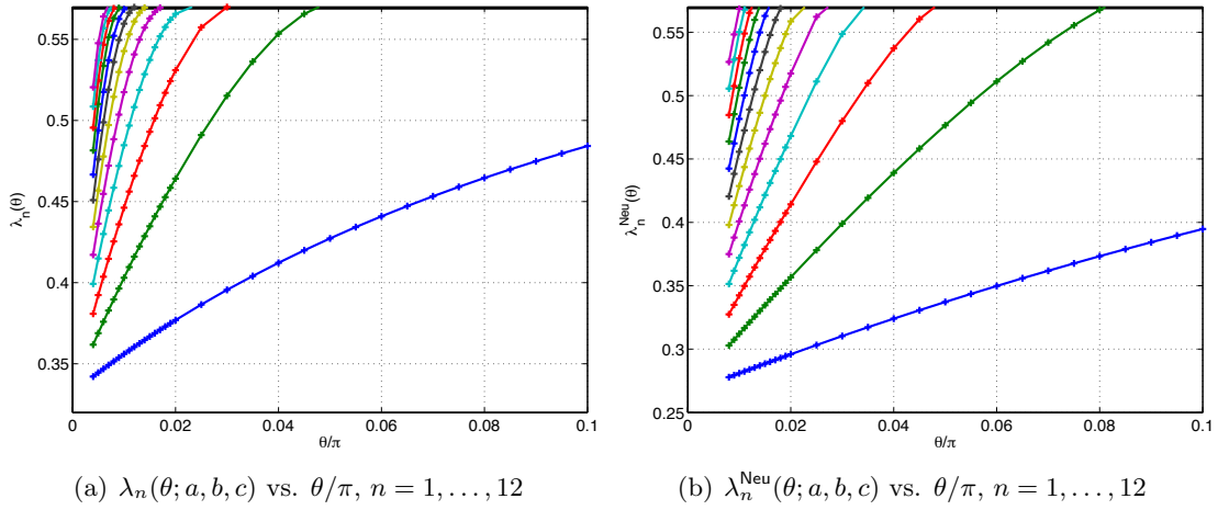
Figure 7: Low lying eigenvalues of \mathcal{L}_\theta (left) and \mathcal{L}_\theta^{\text{Neu}} (right)
