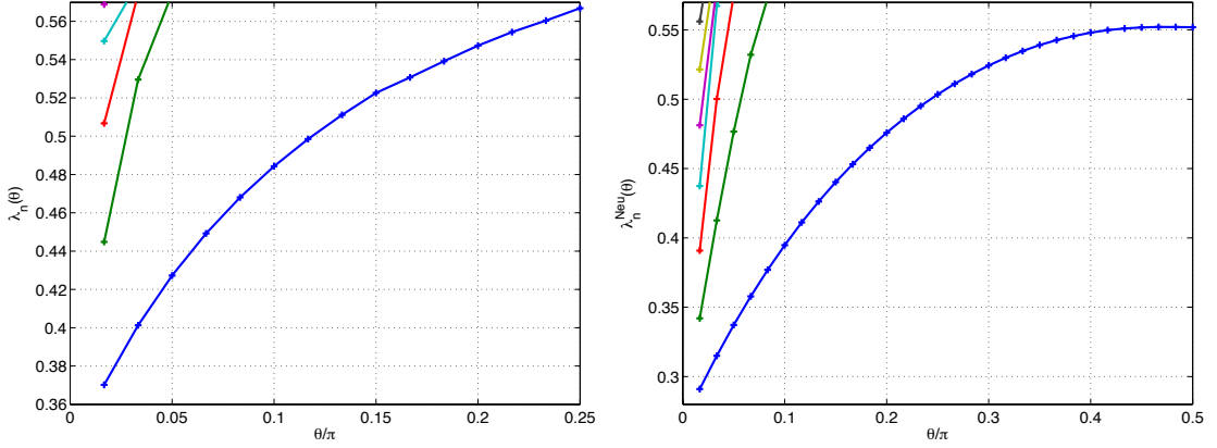
Figure 6: Bottom of the spectrum of \mathcal{L}_\theta (left) and \mathcal{L}_\theta^{\text{Neu}} (right)
