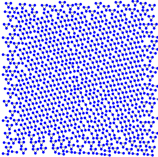
FIGURE 8. A random graph of size n = 1171 with component size at most 3. Observe that most components have size 3, so that the root component is very likely to have size 3.
