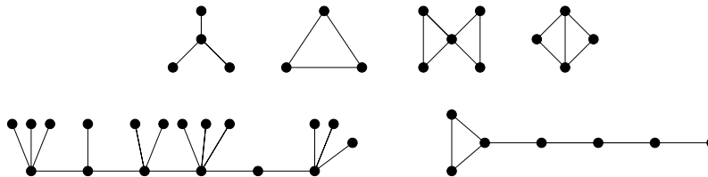
FIGURE 1. A zoo of graphs. Top: the 3-star, the triangle K_3 , the bowtie and the diamond. Bottom: A caterpillar and the 4-spoon (a k -spoon consists of a “handle” formed of k edges, to which a triangle is attached).
