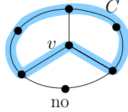
FIGURE 13. A cycle C with an external vertex v of degree at least 3. The cycle shown in gray/blue has a chord that is not short, the contraction of which gives a bowtie.
