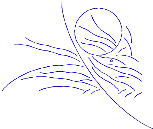
FIGURE 10. A random graph of size n = 1034 avoiding the 3-star.
