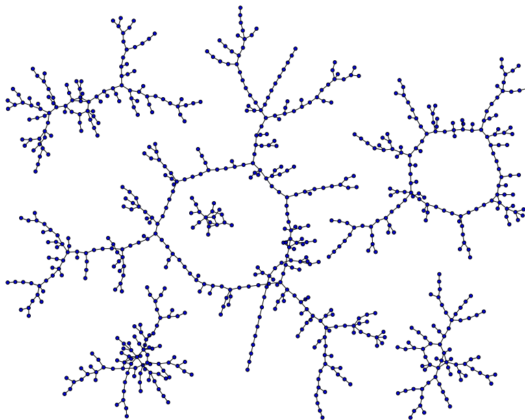
FIGURE 11. A random graph of size n = 758 avoiding the bowtie.
