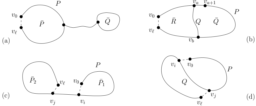
FIGURE 3. A core having several cycles and avoiding the k -spoon cannot contain a path of length 3k - 1 .
