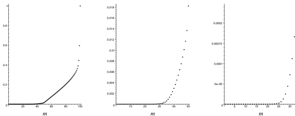
FIGURE 7. The distribution function \mathbb{P}(L_n < m) for n = 100 . The first plot shows the change of regime at m = n/2 , the second the change at m = n/3 , the third the change at m = n/4 .
