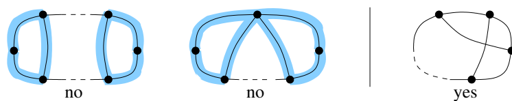
FIGURE 12. The relative positions of two (short) chords in a cycle. The first two configurations are not valid, as these graphs contain a bowtie (shown with gray/blue edges).
