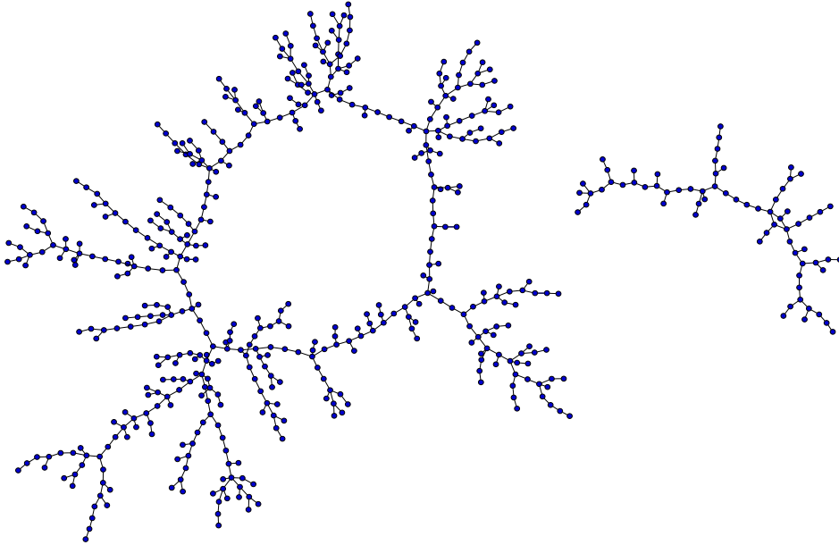
FIGURE 4. A random graph of size n = 541 avoiding the diamond, the bowtie and the 20-spoon.
