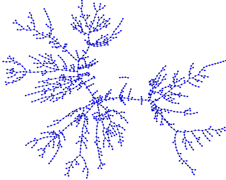
FIGURE 2. A random forest of size n = 1165 . It has two connected components.
