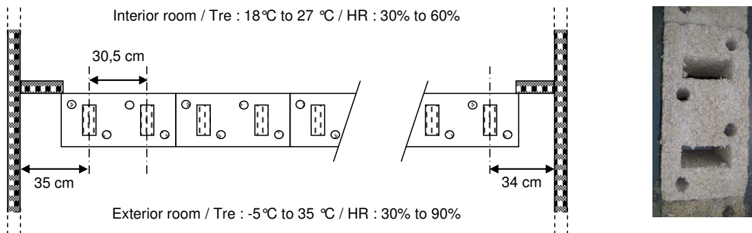
FIG 2 : Wall configuration and hemp concrete block picture
