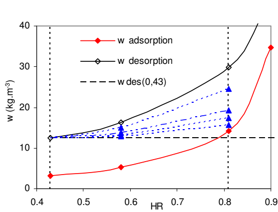
FIG 6 : Intermediate sorption curves for initial water content of w = w_{des}(0.43)
