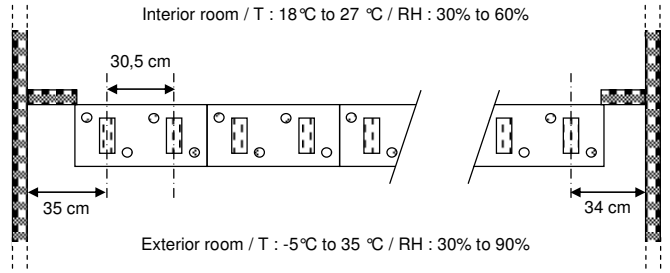
Fig. 1. Wall configuration
