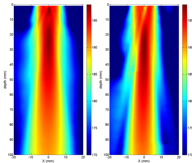
Figure 4: Experimental pressure fields (dB ref 1 \mu Pa) for the primary frequencies at 0.86 MHz (left) and 1.14 MHz (right).
