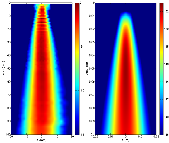
Figure 6: Normalized experimental pressure field (dB) (left) and theoretical pressure field (dB ref 1 μPa) (right) for the parametric frequency (285 kHz).
