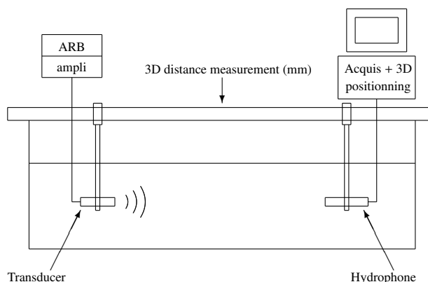
Figure 1: Experimental configuration
