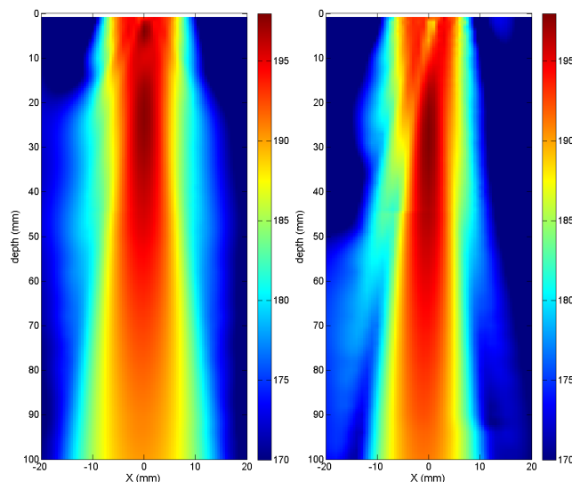
Figure 4: Experimental pressure fields (dB ref 1 \mu\text{Pa} ) for the primary frequencies at 0.86 MHz (left) and 1.14 MHz (right).
