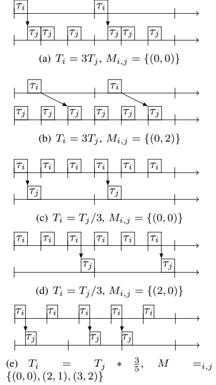
Figure 4. Periodic extended precedence \tau_i \xrightarrow{M_{i,j}} \tau_j
