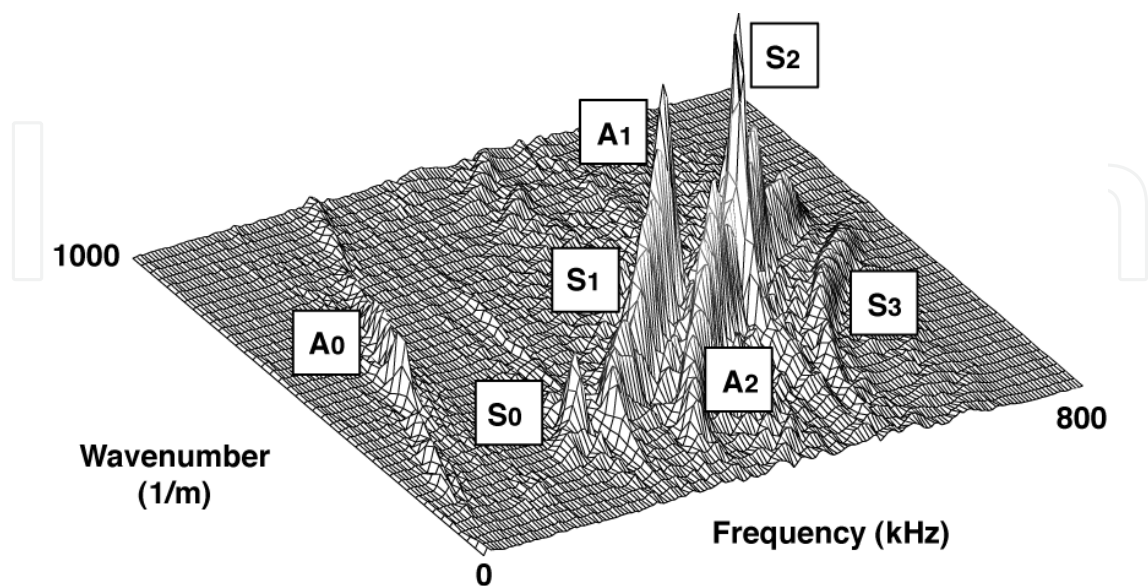
Figure 5. Measurements of the experimental Lamb wave numbers
