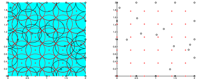
Fig. 2. With the grid addition method.
