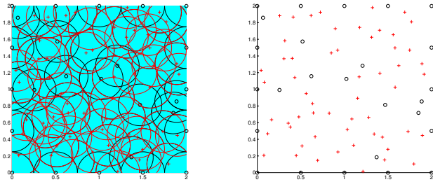
Fig. 4. With the determinantal addition method with a Ginibre basis.
