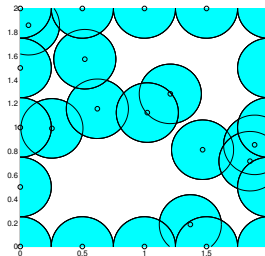
Fig. 1. A damaged wireless network with a fixed boundary.
