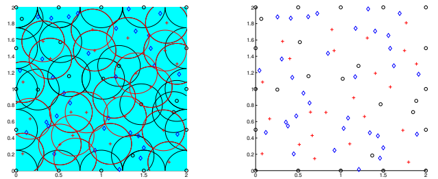
Fig. 5. The reduction algorithm run on the determinantal method example.
