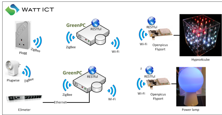
Fig. 1. Schema of the Watt-ICT platform
