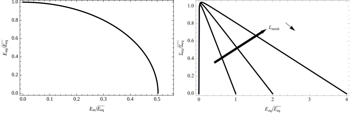
Figure 6: The elliptic damage model (21) (left) and the normalized overall behaviour for a deviatoric applied loading given different values of the mesh size L_{\text{mesh}} (right). The material and cohesive parameters are given in Table 1 and the overall stiffness reduction is tolerated at 5%, i.e. we admit that cohesive zone models disturb the overall Young modulus for less than 5%: E^{\text{hom}}/E^M = 0.95 .
