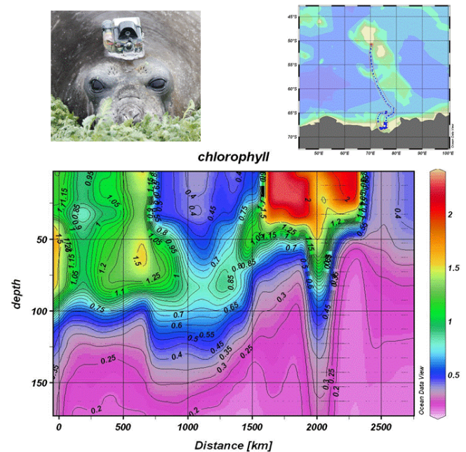
Figure 7. Top: female SES equipped with a CTD-FLUO-SRDL and section to the track followed by a juvenile SES female between January–April 2009. This female left Kerguelen on 12 January and reached the Antarctic shelf on 6 February. This female left the Antarctic shelf on 14 March, the female then remained associated with the marginal ice zone and the Antarctic divergence. Bottom: interpolated quenching corrected fluorescence profiles provided by this SES along its track. This tag exhibited a fluorescence offset of 0.2 \mu\text{g L}^{-1} of chl a and Antarctic values higher than 2 \mu\text{g L}^{-1} were saturated. The abrupt change in chl a concentration (km 2400) coincides with sea-ice formation which took place in mid march. These data show both the latitudinal change in the phytoplankton concentration along a north south transect performed during the inward trip (i.e., 1600 km south of Kerguelen 500 m isobath) and the transition in phytoplankton concentration in Antarctic waters from summer to fall (from km 1600 to 2400).
