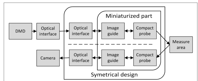
Figure 1. Schematic representation of the 3D measurement system.
