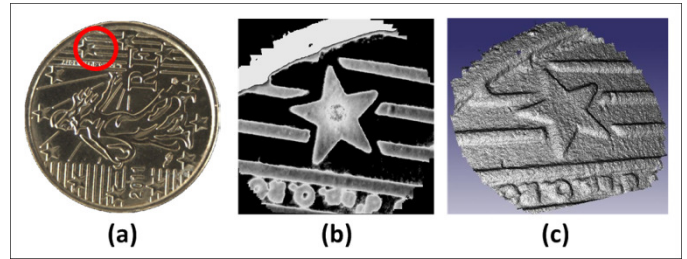
Figure 3. (a) Measurement area on the 10 cent euro coin. (b) Depth map of the measured surface. (c) 3D reconstructed surface
