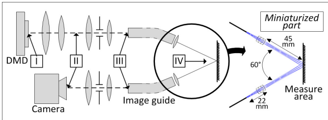
Figure 2. Optical elements of the 3D measurement system
