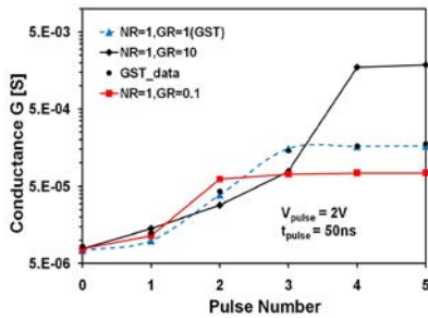
Fig.6 Simulated LTP curves while fixing the nucleation rate (NR) and varying the growth rate GR compared to GST (reference: GR=1, NR=1). Corresponding simulations of PC layer morphology is shown (0 th pulse: reset; 1 st -5 th : potentiating).
