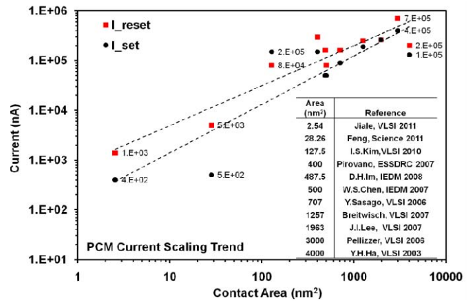
Fig.17 Scaling trend of Reset and Set current for different PCM technologies. Set current values are extracted from literature. Interpolations are also shown
