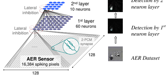
Fig.9 Topological overview of the spiking neural network
