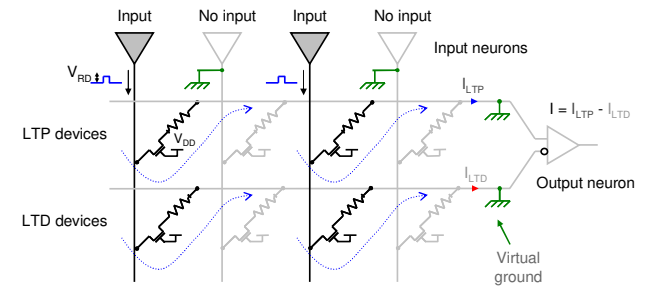
Fig.12 Read circuit scheme. Current from both LTP and LTD PCM devices is integrated in the output neuron, with a positive and negative contribution, respectively.
