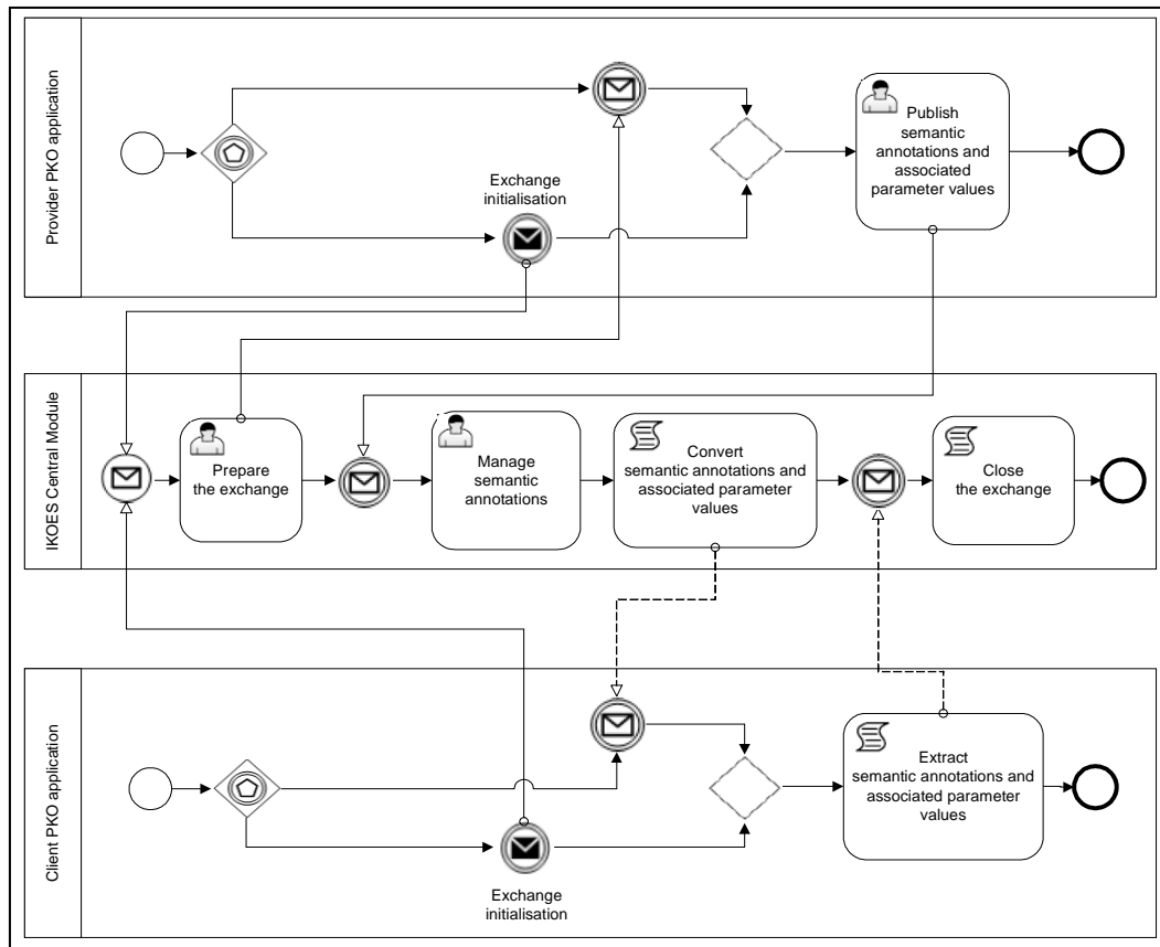
Figure 9. Inter-knowledge objects exchange process model
