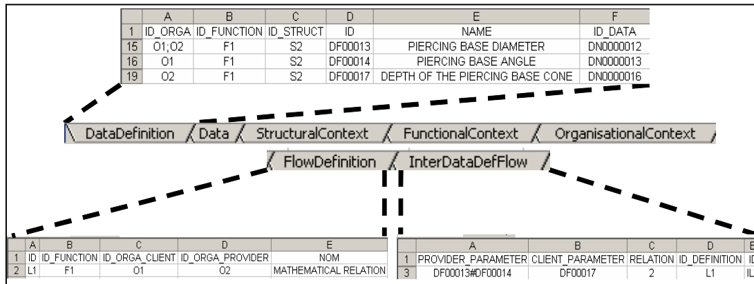
Figure 13. Extract from the Excel dictionary file
