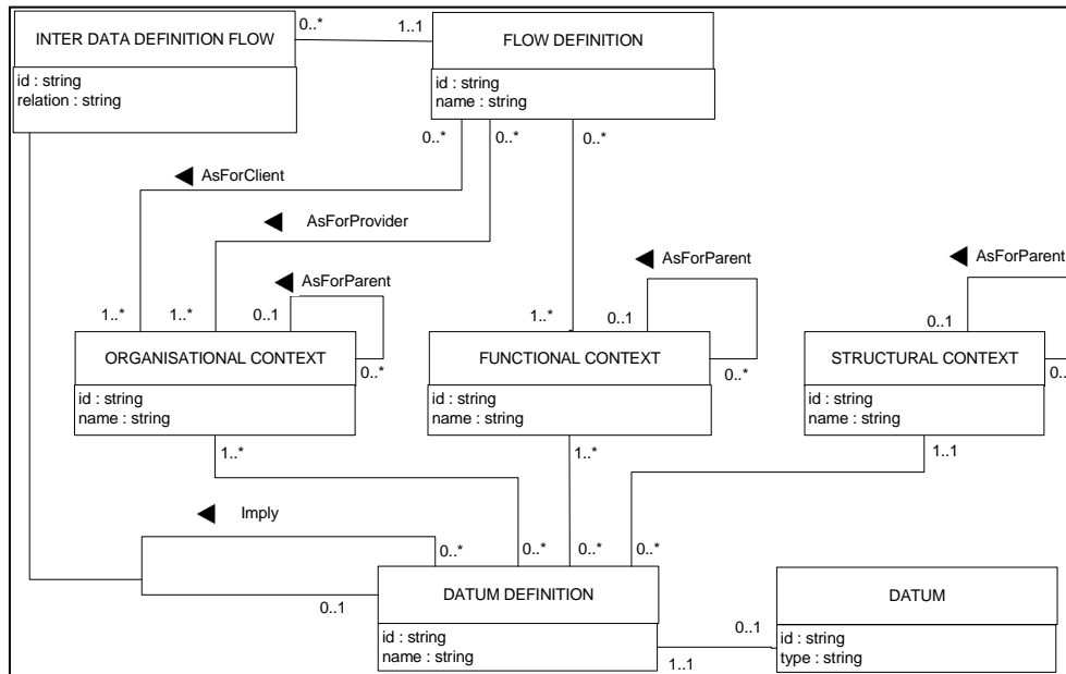
Figure 3. Data structure model
