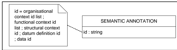
Figure 5. Data model
