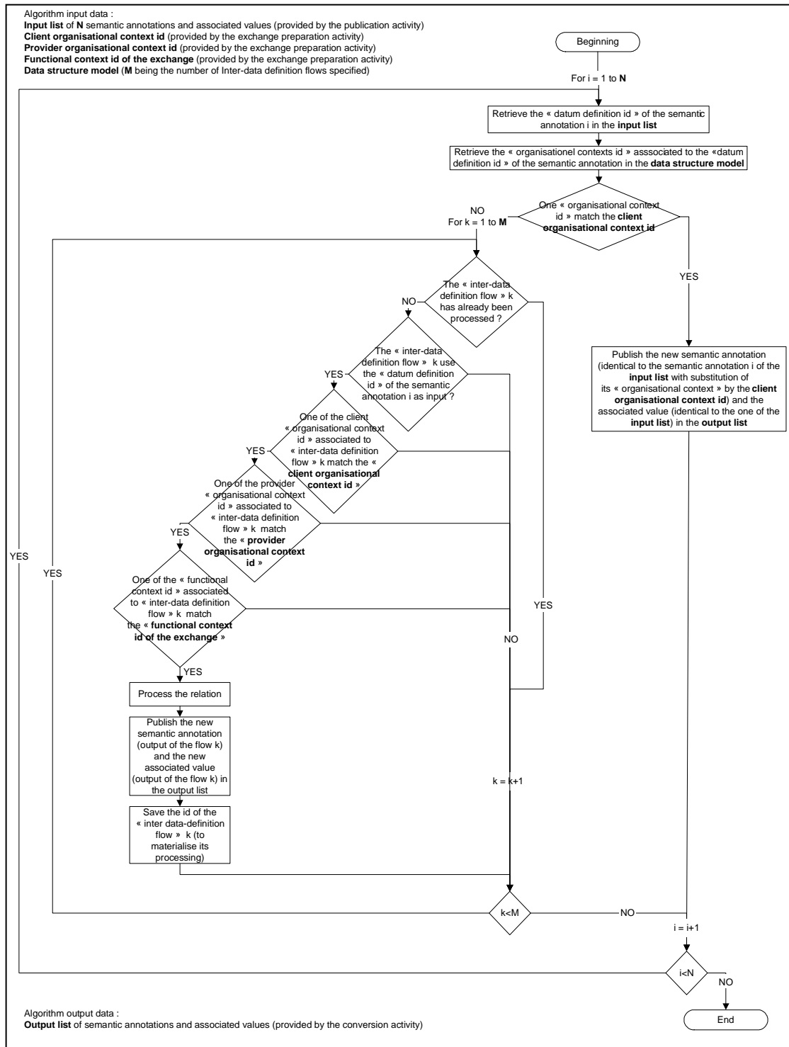
Figure 8. Conversion algorithm for semantic annotations and related parameter values
