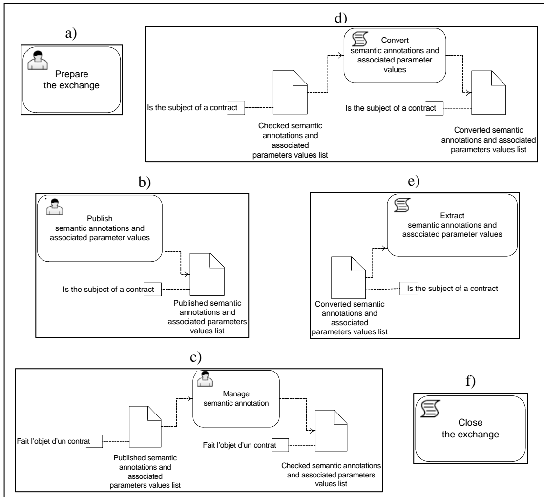
Figure 7. Inter-knowledge objects exchange activities model
