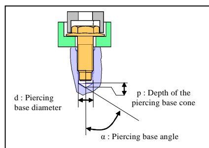
Figure 1. Description of three parameters of a screwed assembly
