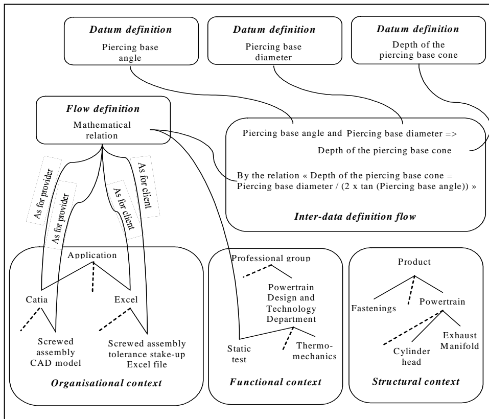
Figure 4. Example of an instance for flow-type knowledge representation between parameters
