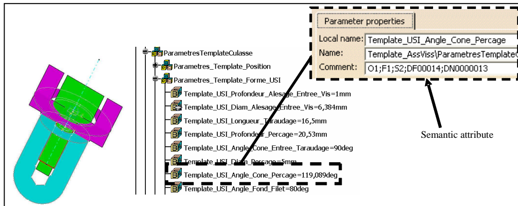
Figure 11. CAD PKO
