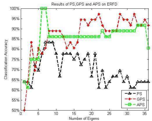
Figure 8 – Classification accuracy of PS, GPS and APS on ERFD.
