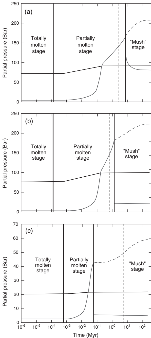
Figure 13. Time evolution of partial pressure of uncondensed \text{H}_2\text{O} (grey line), total \text{H}_2\text{O} (grey dashed line) and \text{CO}_2 (black line) for (a) Venus, (b) the Earth, and (c) Mars. Condensation of water vapor occurs at the end of the magma ocean phase ( t_c = t_p ). It corresponds to the beginning of the mush stage shown by the vertical lines on the figure. For comparison, we also draw a dashed line corresponding to a threshold of 98% solidification in volume (grey line) [Elkins-Tanton, 2008]. Parameters used for the calculations are given in Table 4.
